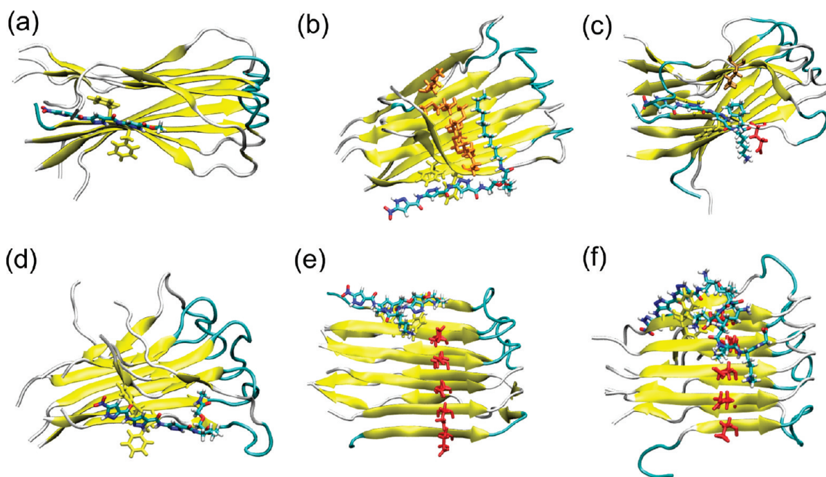
Figure 2. Final complex structures resulting from 20 ns molecular dynamics simulations of different C-terminally extended aminopyrazole ligands (cpk coloring) in complex with a pentameric Aβ 42 -protofilament. Interacting residues are shown in stick representation: Phe19/20 (yellow), Glu22 (red), and Met35 (orange). (a) Trimer-OMe, (b) Trimer-TEG-Dd, (c) Trimer-K-Che, (d) Trimer-TEG-NHMe, (e) Trimer-TEG-K, and (f) Trimer-TEG-KKKKKG-OH.
