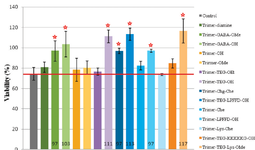
Figure 7. Viability assays of PC-12 cells with trimeric aminopyrazoles ( 100 \mu\text{M} ). \text{A}\beta lesion control ( 10 \mu\text{M} ) was set at \sim 75\% viability. Most effective drugs are marked with asterisks.
