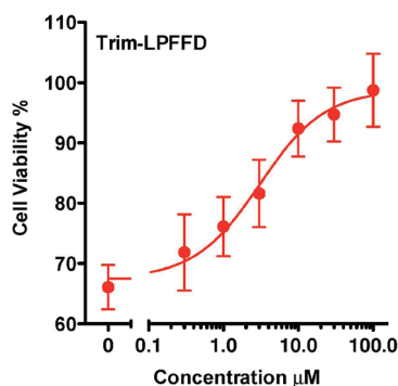
Figure 8. Dose-response curve for inhibition of \text{A}\beta -induced toxicity in PC-12 cells by Trimer-LPFFD ( \text{IC}_{50} = 3.1 \mu\text{M} ).
