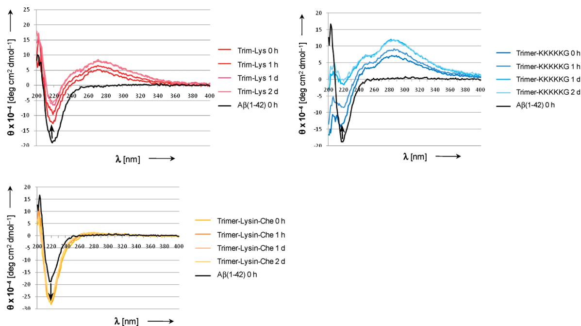
Figure 6. Typical CD spectra recorded for aggregated A \beta (1–42) alone (black) and after addition of aminopyrazole ligand (type A, Trimer-K-OMe: red; type B, Trimer-KKKKKG-OH blue; type C, Trimer-K-Che: brown). Time progresses in the direction of the embedded arrows, indicated by lighter colors (0 h, 1 h, 1 d, 2 d). Test solutions contained 10 \mu M A \beta (1–42), 5 \mu M potassium phosphate buffer (pH = 7.3), 2% HFIP, and 10 \mu M of the respective aminopyrazole trimer derivative.
