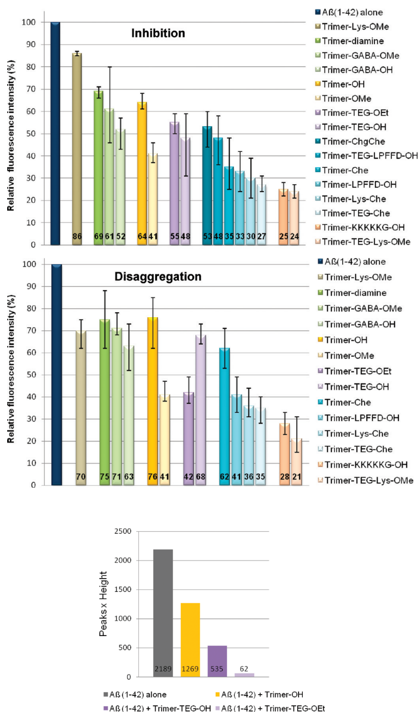
Figure 4. Equilibrium of 33 \mu\text{M} \text{A}\beta_{42} aggregation vs disaggregation in the absence or presence of trimeric aminopyrazole inhibitors (each at 198 \mu\text{M} ): (top) inhibition of aggregation and (middle) disaggregation (10 mM PBS, pH 7.3). The color code for each aminopyrazole trimer derivative is maintained throughout the entire article. For each bar 6 measurements were averaged. (Bottom) FCS measurements at 5 nm \text{A}\beta with Trimer-OH in comparison to Trimer-TEG-OH/OEt (each at 100 nM).
