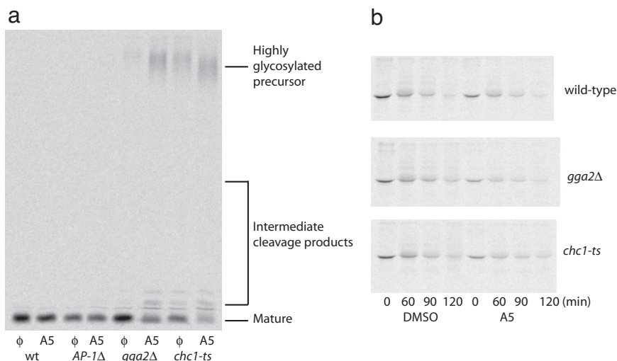
Fig. 3. Compound A5 specifically inhibits AP-1-dependent traffic. (a) Synthetic α-factor maturation defects caused by A5. Cells of the indicated genotype (same strains as in Fig. 2a) were treated with compound, and α-factor was analyzed as in Fig. 2b. (b) Degradation of Ste3p is not affected by compound A5 treatment. Cells were treated and labeled as in Fig. 2b, and Ste3p was immunoprecipitated at the indicated chase points from cell lysates and visualized by SDS/PAGE and autoradiography.
