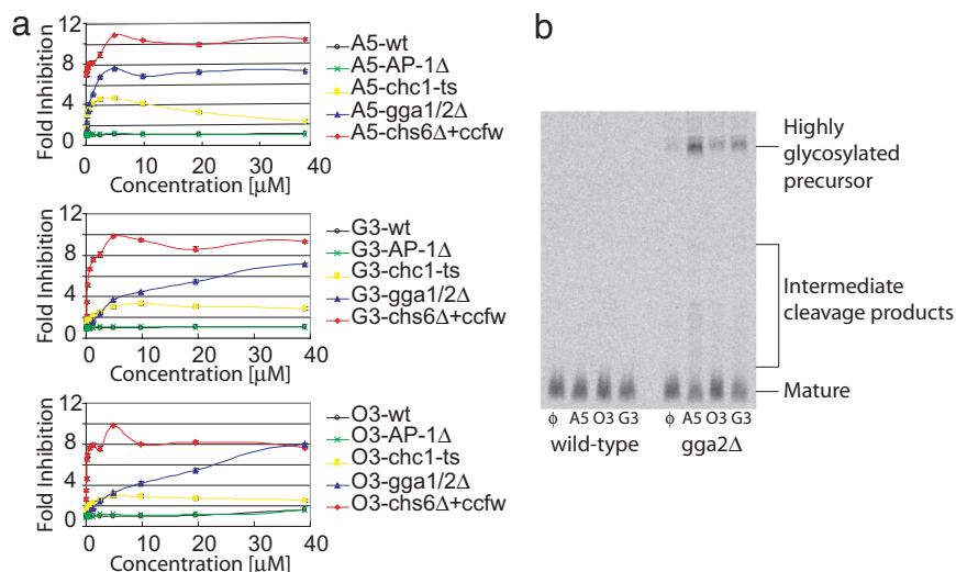
Fig. 2. Synthetic growth and traffic inhibition by CSL active compounds. (a) Synthetic growth effects. Compounds A5 (Top), G3 (Middle), and O3 (Bottom) were added at different concentrations to wild-type (MDY326), AP-1Δ ( apl2Δ apl4Δ ; MDY334), chc1-ts (MDY330), and gga1/2Δ (MDY327) cells, or chs6Δ (MDY335) cells with 60 μM ccfw. Values represent the fold growth inhibition observed after overnight incubation with compound compared with growth of the same strains with DMSO. (b) Synthetic effects on α-factor maturation. Wild-type (MDY326) or gga2Δ (MDY380) cells were treated with indicated compounds (25 μM) or DMSO (Φ) overnight, metabolically labeled for 10 min, and subjected to a 30-min chase. Secreted α-factor was immunoprecipitated from the media and imaged by SDS/PAGE followed by autoradiography.
